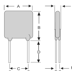
Figure 3 FRK135-60F~FRK500-60F Lead Size : 20AWG Φ 0.81 mm Diameter
