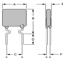
Figure 2 FRK110-60F Lead Size : 20AWG Φ 0.81 mm Diameter
