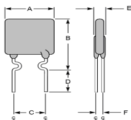
Figure 1 FRK050-60F~FRK090-60F Lead Size :24AWG Φ 0.51 mm Diameter
